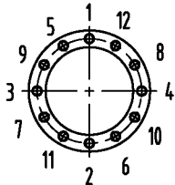
胀紧套螺栓预紧顺序
